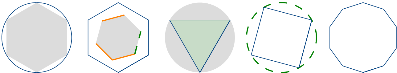
Regular polygon examples
